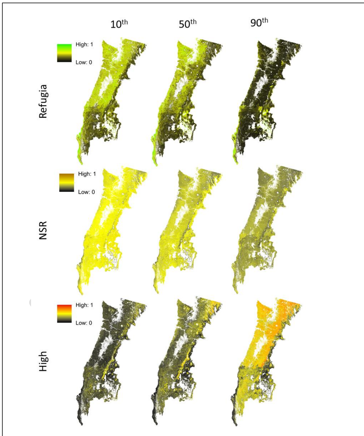
Figure 8. Probability surface maps of fire refugia, NSR severity, and high-severity under low (10 th percentile), moderate (50 th percentile), and extreme (90 th percentile) fire growth and weather conditions over the period 2001-2017 and 1986-2018, respectively. DAB and RMIN were the two top time-varying predictors in these model runs.
