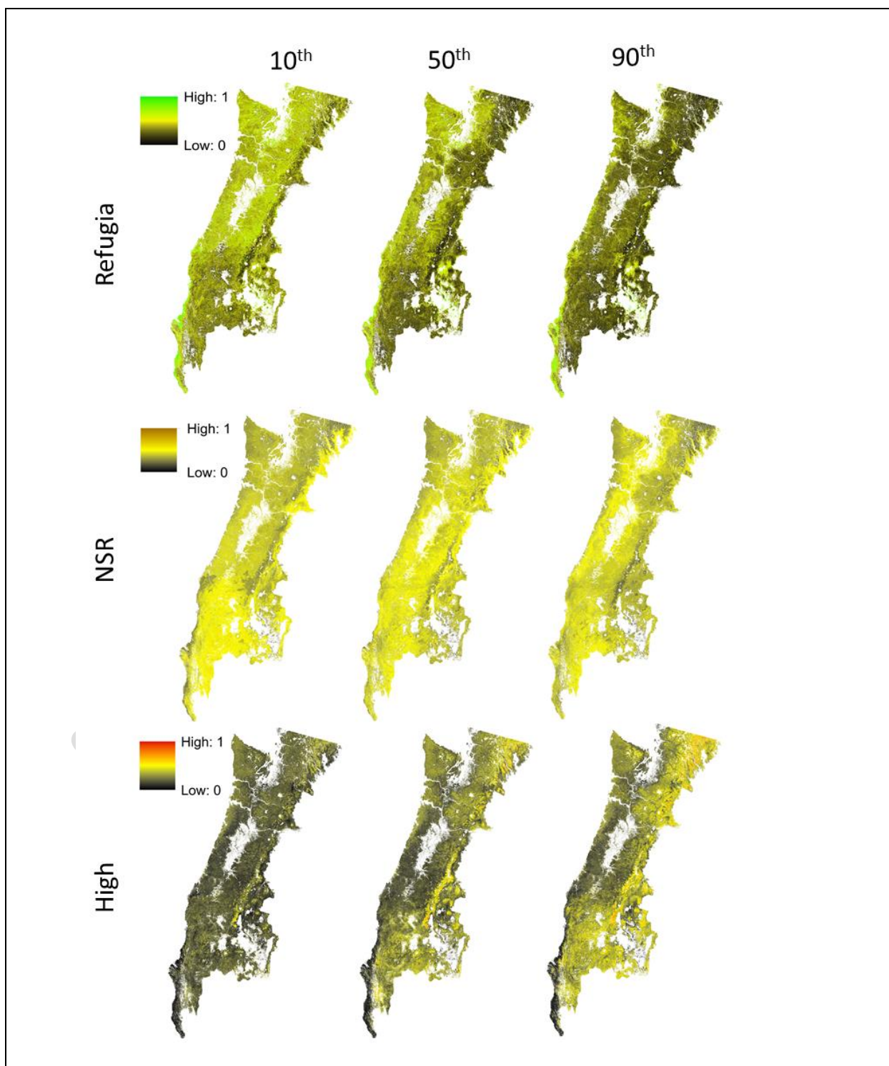
Figure 7. Probability surface maps of fire refugia, NSR severity, and high-severity under low (10 th percentile), moderate (50 th percentile), and extreme (90 th percentile) fire weather conditions over the period 1986-2018 based on models with no fire growth term. Fire weather scenarios were driven by TMMX and RMIN, the most consistently ranked top fire weather variables across all model runs, except for NSR models, where FM1000 was used in place of TMMX.
