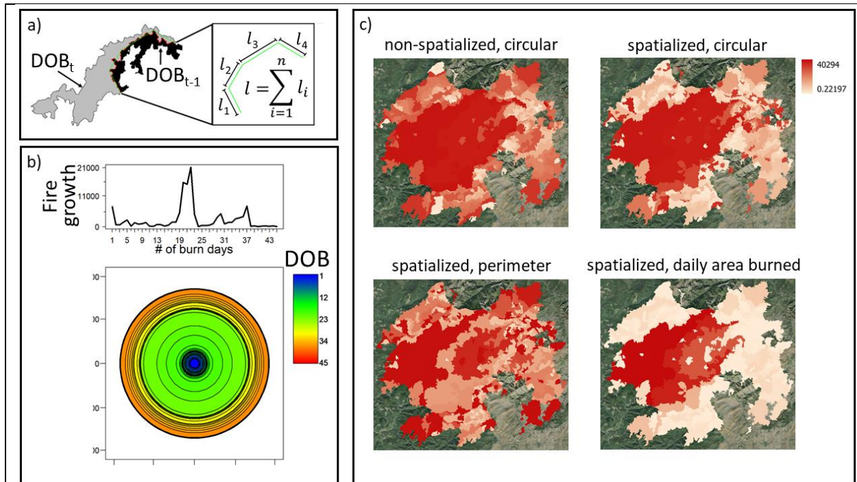
Figure 3. Fire growth characterization methods and outputs derived from analysis of daily fire progression maps. Panel (a) shows the daily fire perimeters for two consecutive days-of-burn, DOB_t and DOB_{t-1} . The inset shows the smoothed estimation method for the perimeter method. Panel (b) shows the non-spatialized circular method for conversion of daily area burned to planar fire growth for the Chetco Bar fire of 2017, along with a time series of the resulting daily fire growth patterns in the line graph above. Panel (c) shows rasters of the non-spatialized circular method (upper left) and spatialized circular (FG_CIRC, upper right), perimeter (FG_P_MEAN, lower left), and daily area burned (DAB, lower right) methods of fire growth characterization for the Chetco Bar fire.
