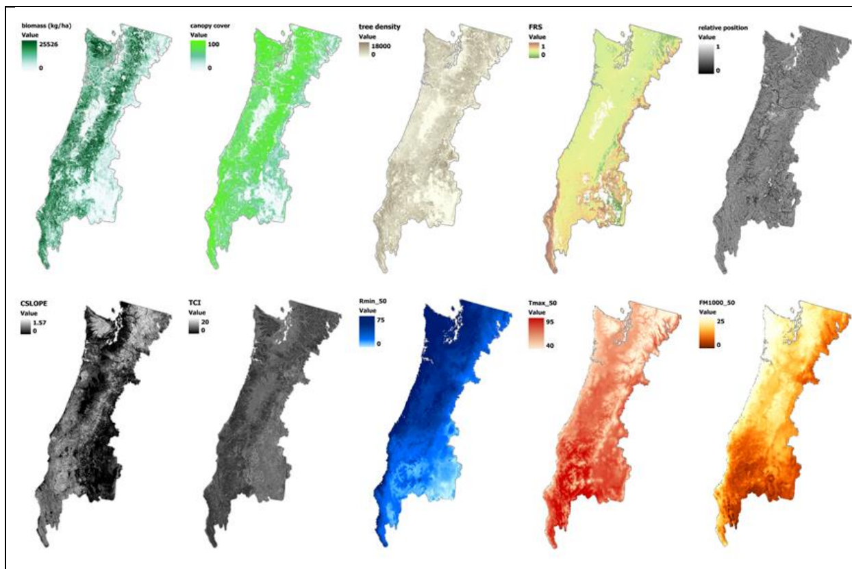
Figure 2. Raster surfaces for many of the top predictor variables in our final models. Note that the fire weather rasters depicted here are the pixel-wise 50 th percentile calculations for time-varying variables used in the fire weather scenarios.
