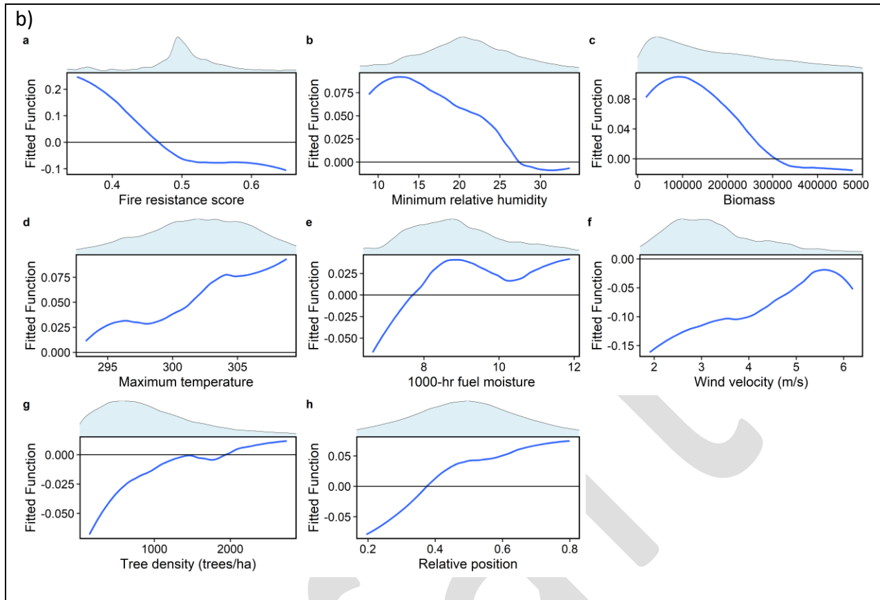
Figure 6. Partial dependence plots for high-severity fire weather models for (a) the non-fire-prone and (b) fire prone ecoregions. Partial dependence plots show the conditional influence of each predictor variable on the high-severity model, while holding all other predictors constant. Density plots above each panel show the data distribution of each predictor in our modeling dataset.
