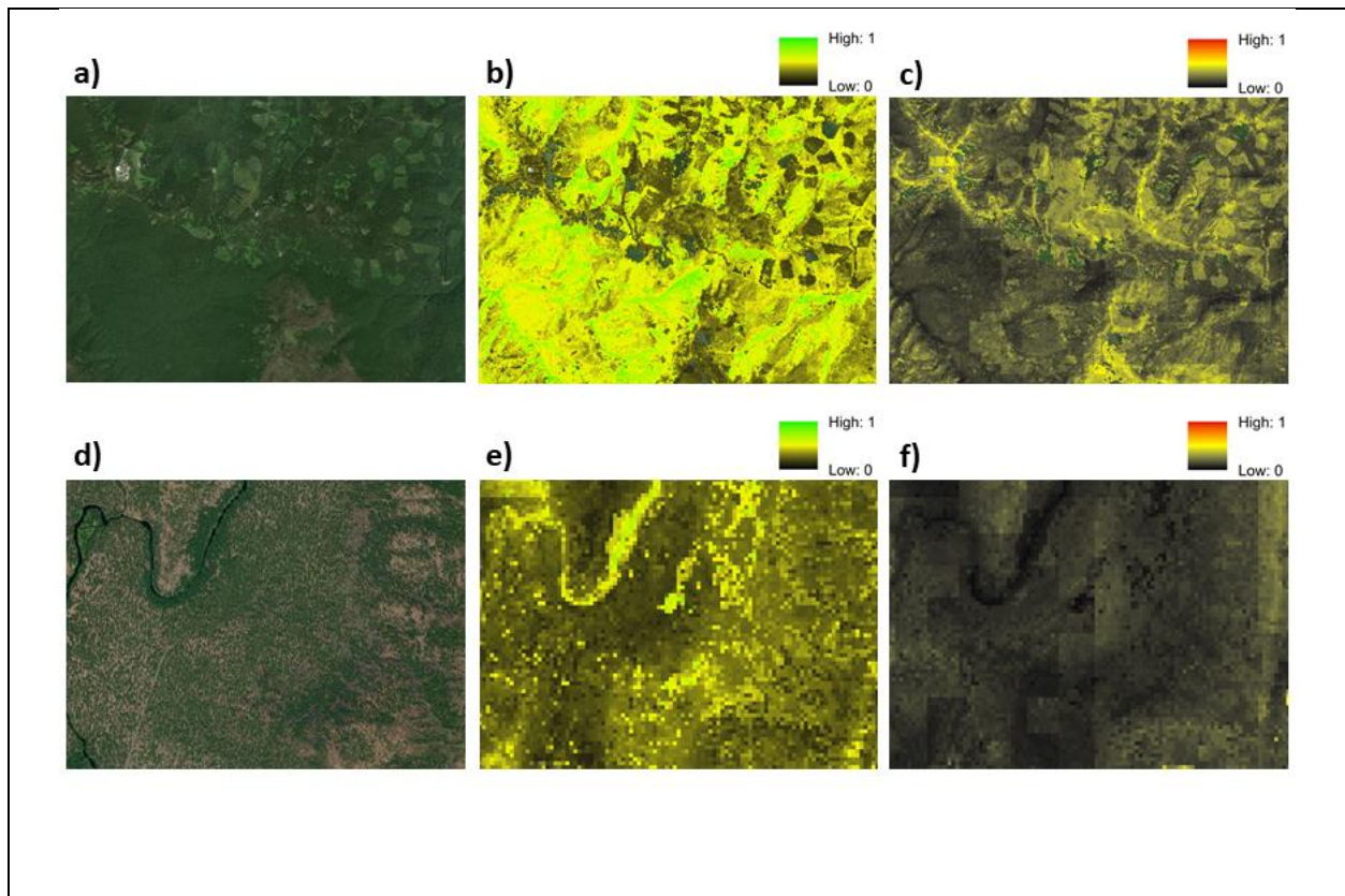
Figure 9. Mid-scale view of an area in the (a-c) non-fire-prone ecoregion and (d-f) fire-prone ecoregion, showing (a,d) an true color satellite image, (b,e) modeled fire refugia, and (c,f) modeled high severity fire probability. In the non-fire-prone ecoregion, note the concentration of refugia along low-lying topographic positions and the long-term reduction of refugial probability resulting from past timber harvest. In the fire-prone ecoregion, note the fine-scale spatial patterning of refugia, the prevalence of intermediate refugial probability, and the low probability of high severity fire.
