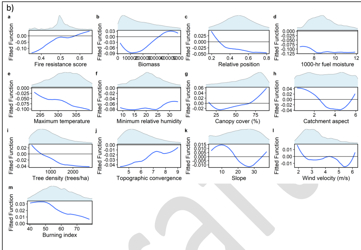
Figure 5. Partial dependence plots for refugia fire weather models for (a) the non-fire-prone and (b) fire prone ecoregions. Partial dependence plots show the conditional influence of each predictor variable on the refugia model, while holding all other predictors constant. Density plots above each panel show the data distribution of each predictor in our modeling dataset.
