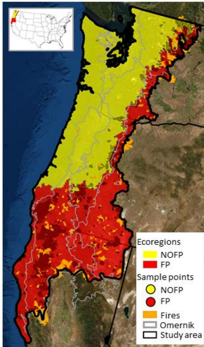
Figure 1. Study area map showing the study extent, ecoregional boundaries, sample pixels used for modeling, and study fires 2002-2017 included in our analysis. EPA level III ecoregions (Omernik 1987) are also displayed for comparison with ecoregions derived for this study.
